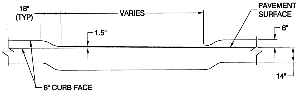
DEPRESSED CURB AT DRIVE APRON
